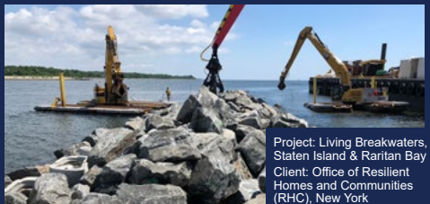
View of breakwater trunk under construction.
