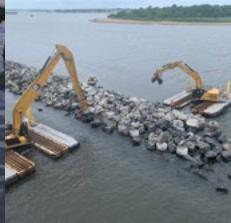
Breakwater crenulation under construction.
