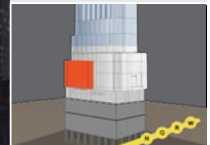
Completed Project with Theater Lifted, Caissons Installed and Additional Cellar Level Constructed
