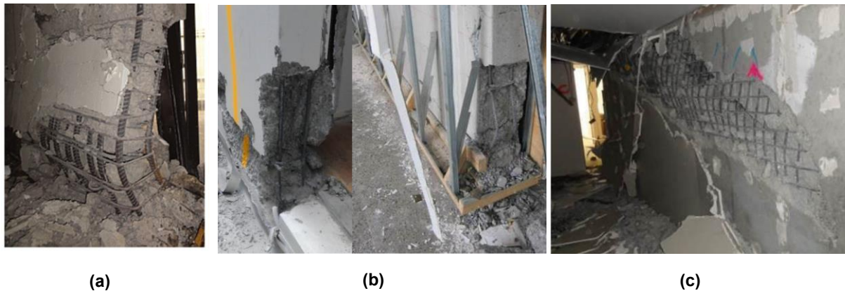
Figure 1. Wall damage in the the 2010-11 Canterbury earthquake sequence: (a) buckling of well-confined wall (Elwood 2013); (b) bar buckling and fracture (Kam et al. 2011); (c) shear-axial failure (Kam et al. 2011)
