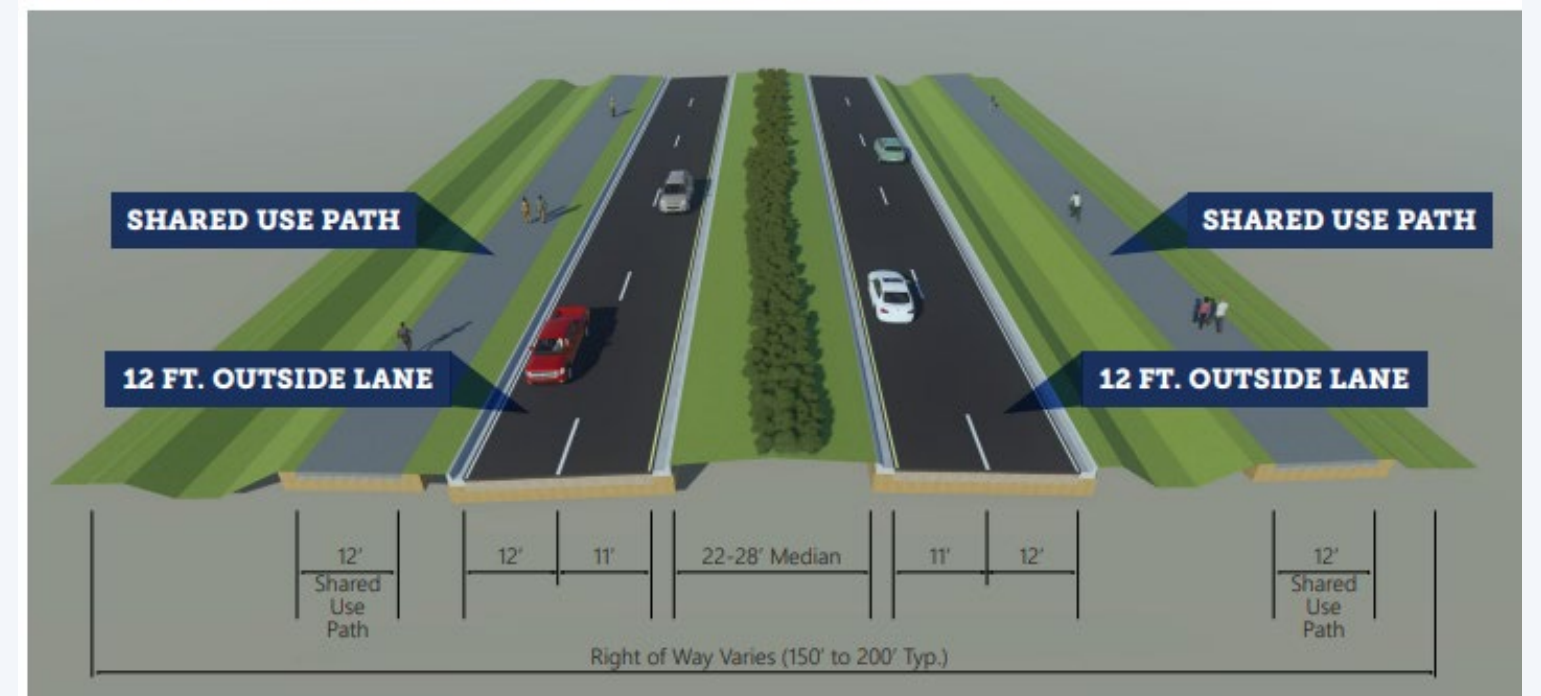
Four Lane Urban Typical (Full Reconstruction)
