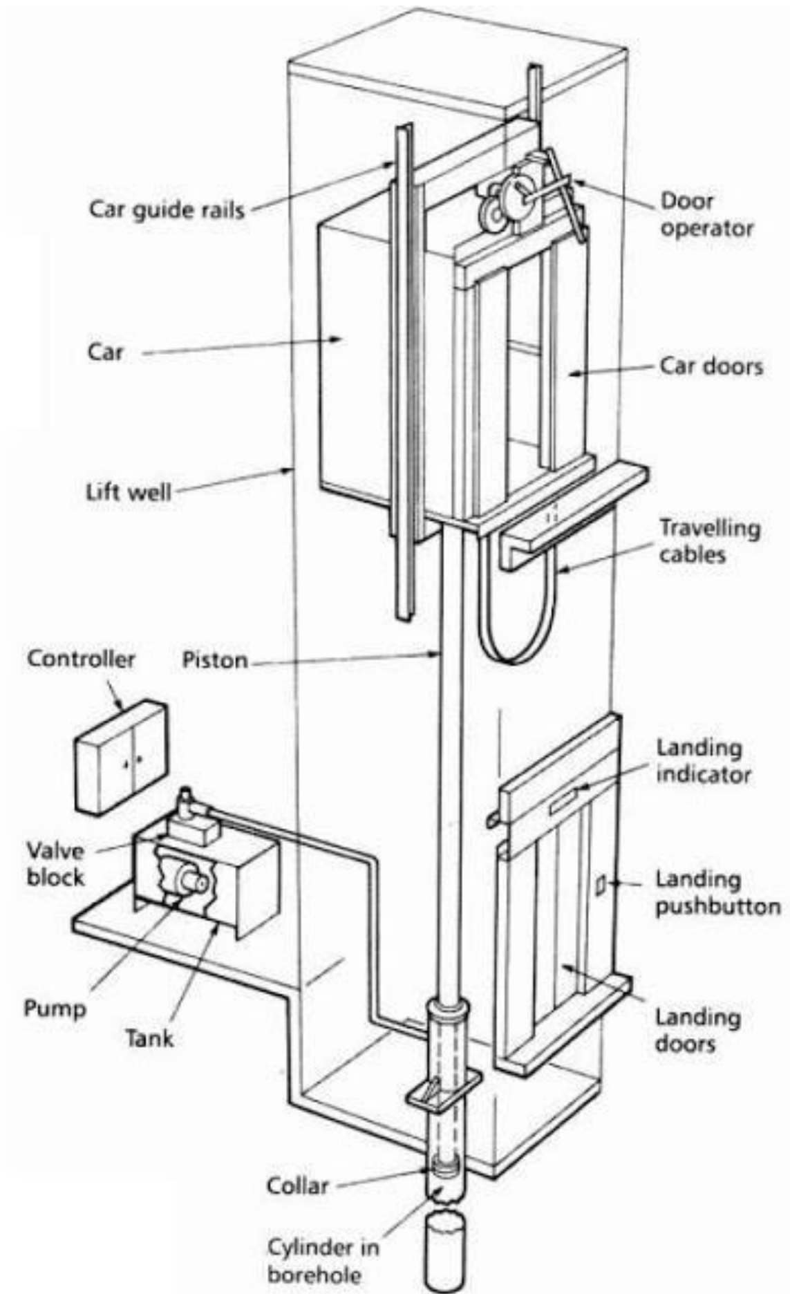
Hydraulic (Low-rise)
