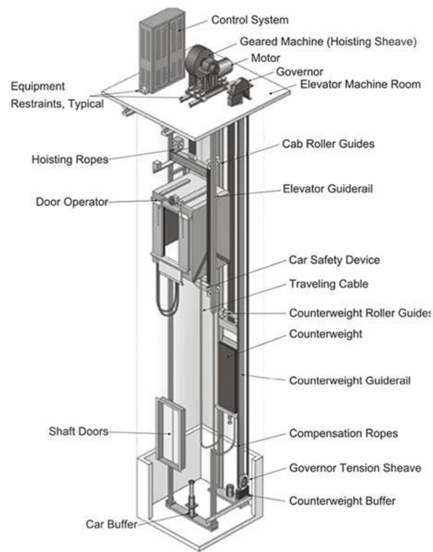
Geared (Mid-rise)
