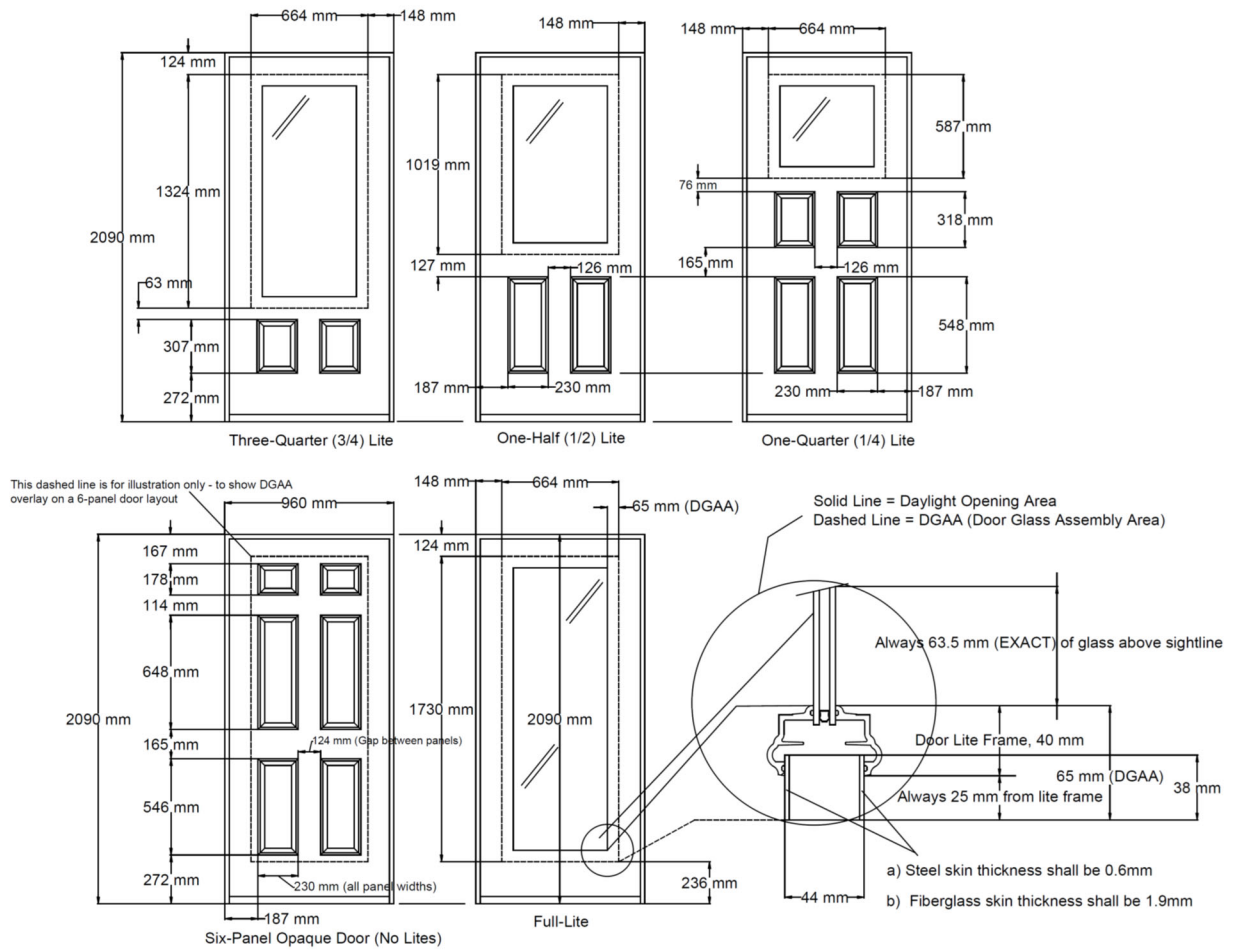
Figure 5-10 – SDR Configurations of Single Door or Sidelights
