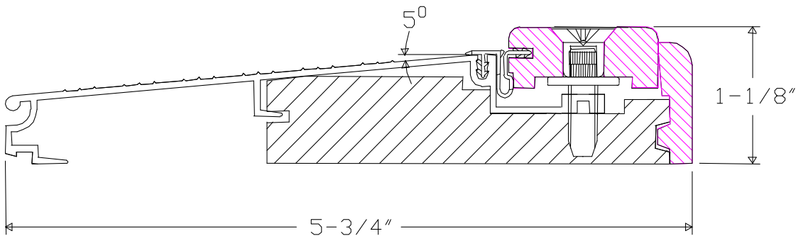
Figure 5-8a – Default Thermally Broken Aluminum Door Sill
