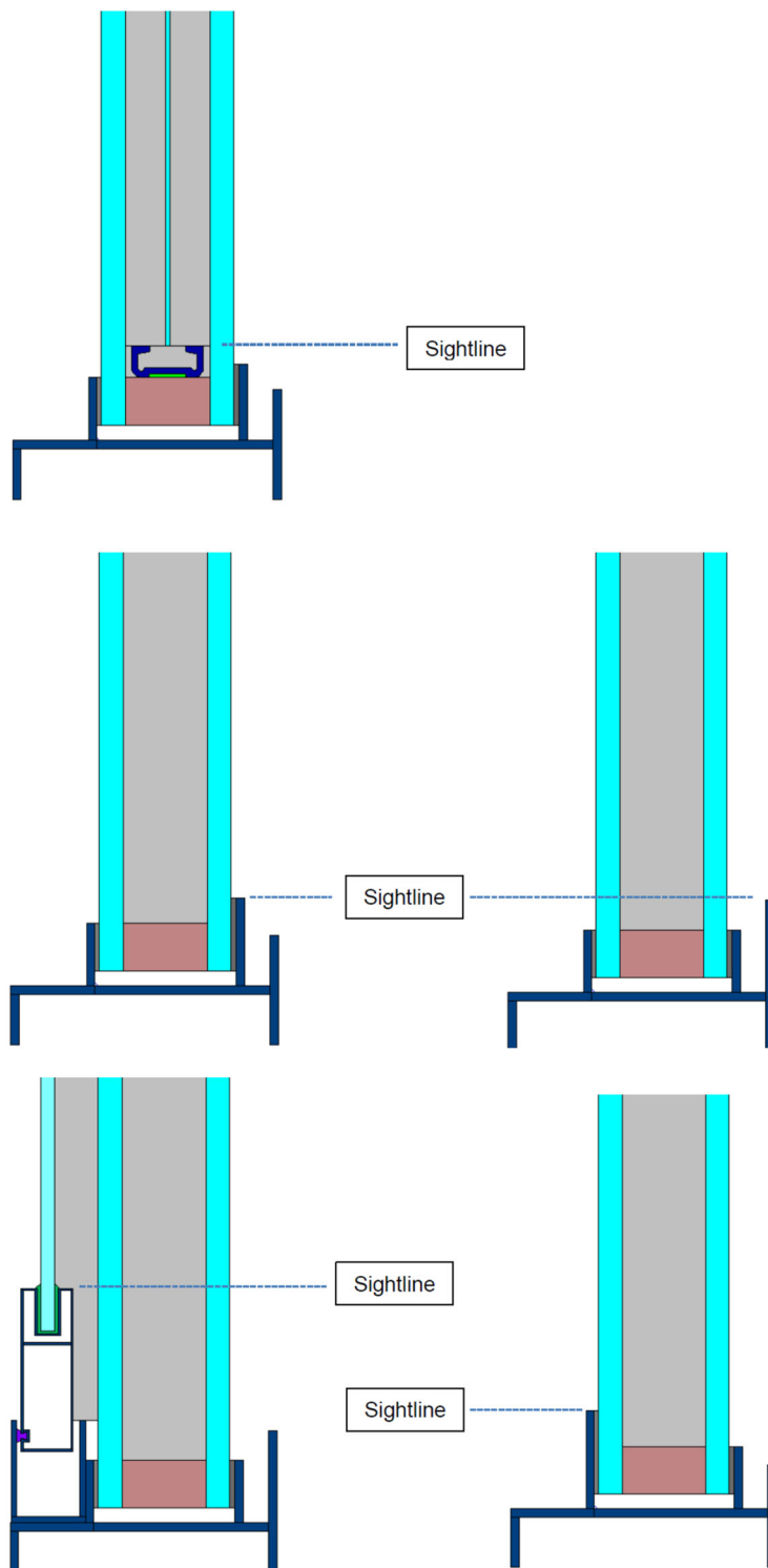
Figure 4-4 – Sightline Examples
