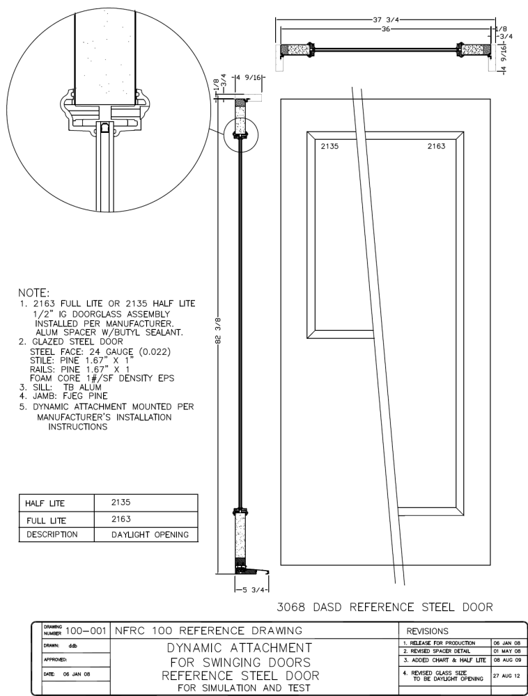
Figure 5-18 – Reference Swinging Door Details
