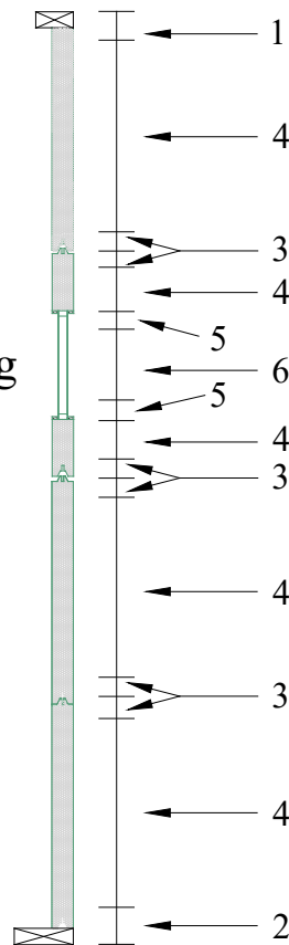
Figure 5-15 – Garage Door U-factor Area Weighting, Sectional
