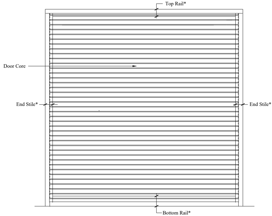
Figure 5-22 – Rolling Door U-factor Area Weighting – Front Elevation View
