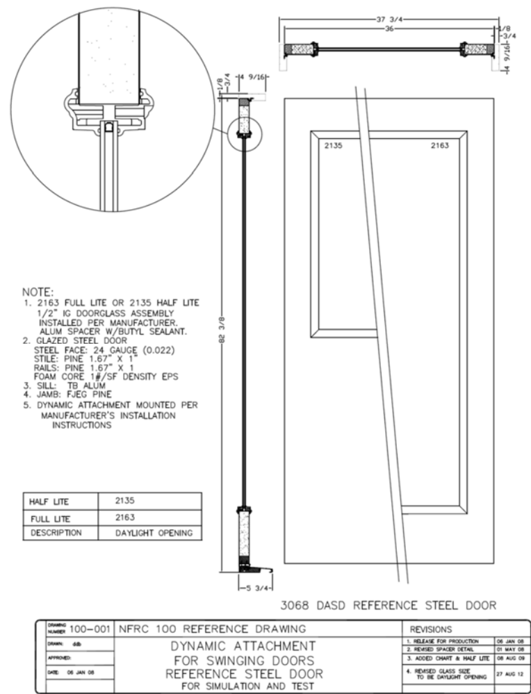
Figure 5-19 – Reference Swinging Door Details
