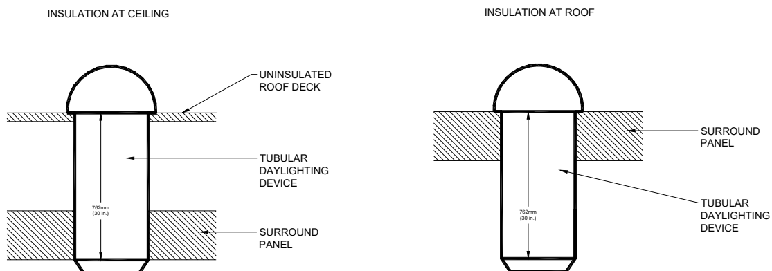
Figure 5-15a – Tubular Daylighting Device Product Schematic – Vertical Elevation
