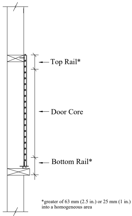
Figure 5-21 – Rolling Door U-factor Area Weighting - Sectional View
