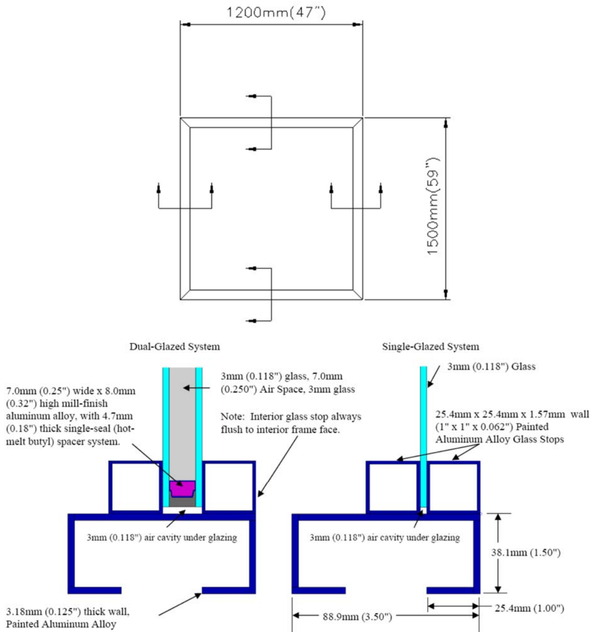
Figure 5-24 – Residential Fixed Window Reference Product
