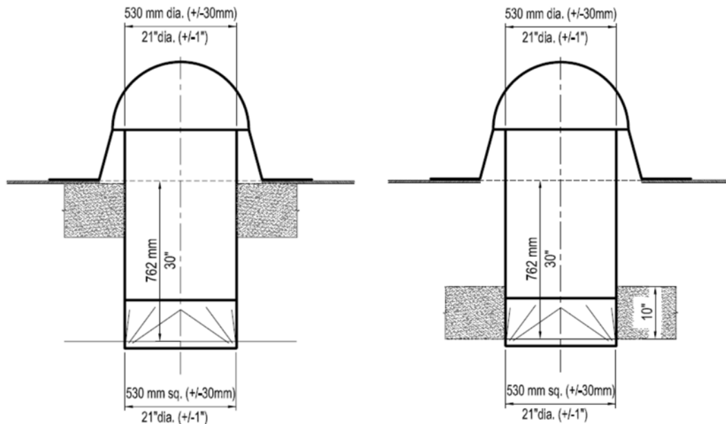
Figure 5-15b – Hybrid Tubular Daylighting Device Product Schematic – Vertical Elevation
