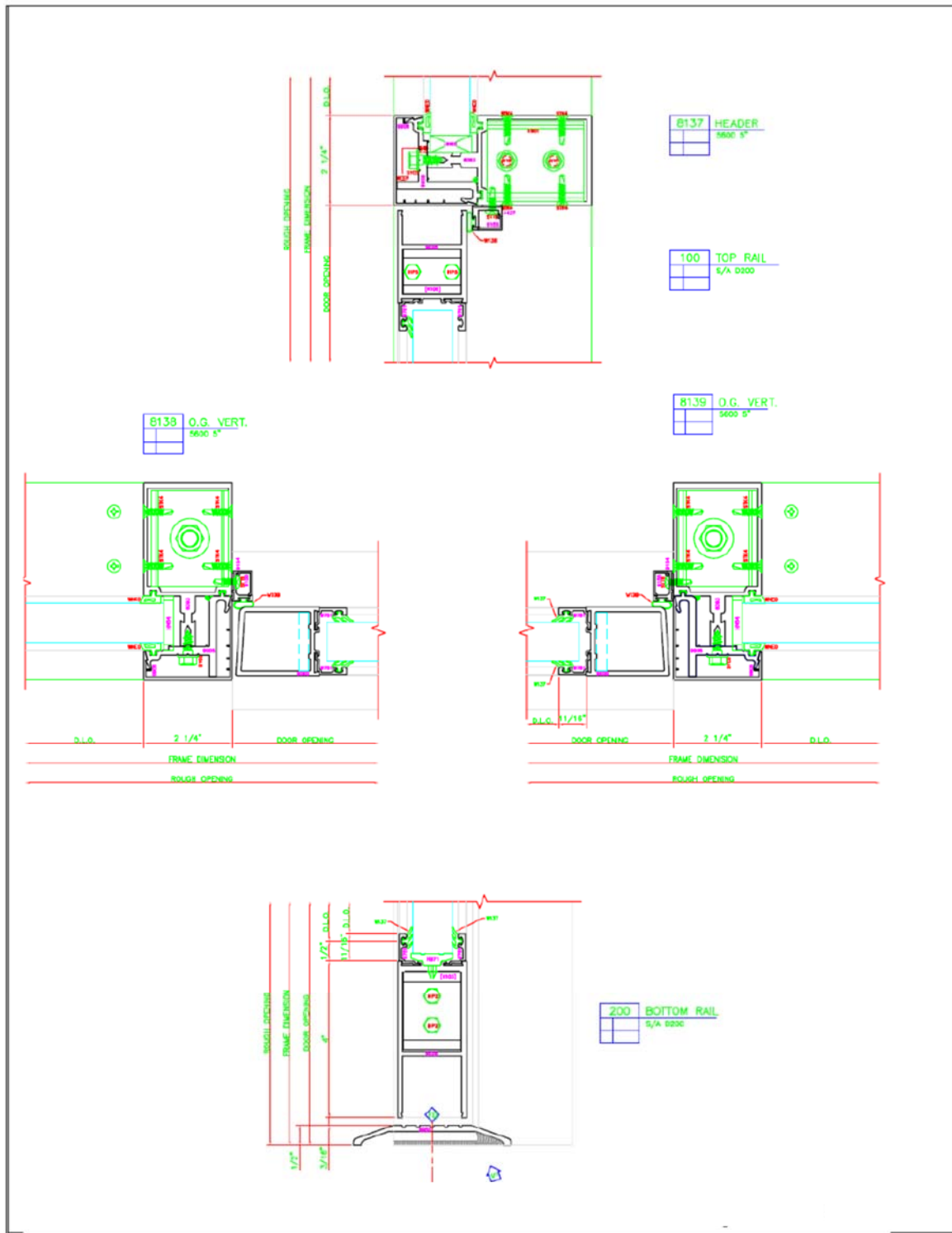
Figure 5-14 – Door Inside Curtainwall Glazed Wall System
