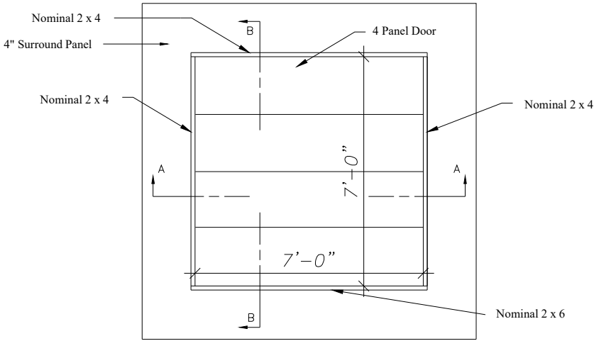
Figure 5-18 – Garage Door Front Elevation View and Perimeter Details
