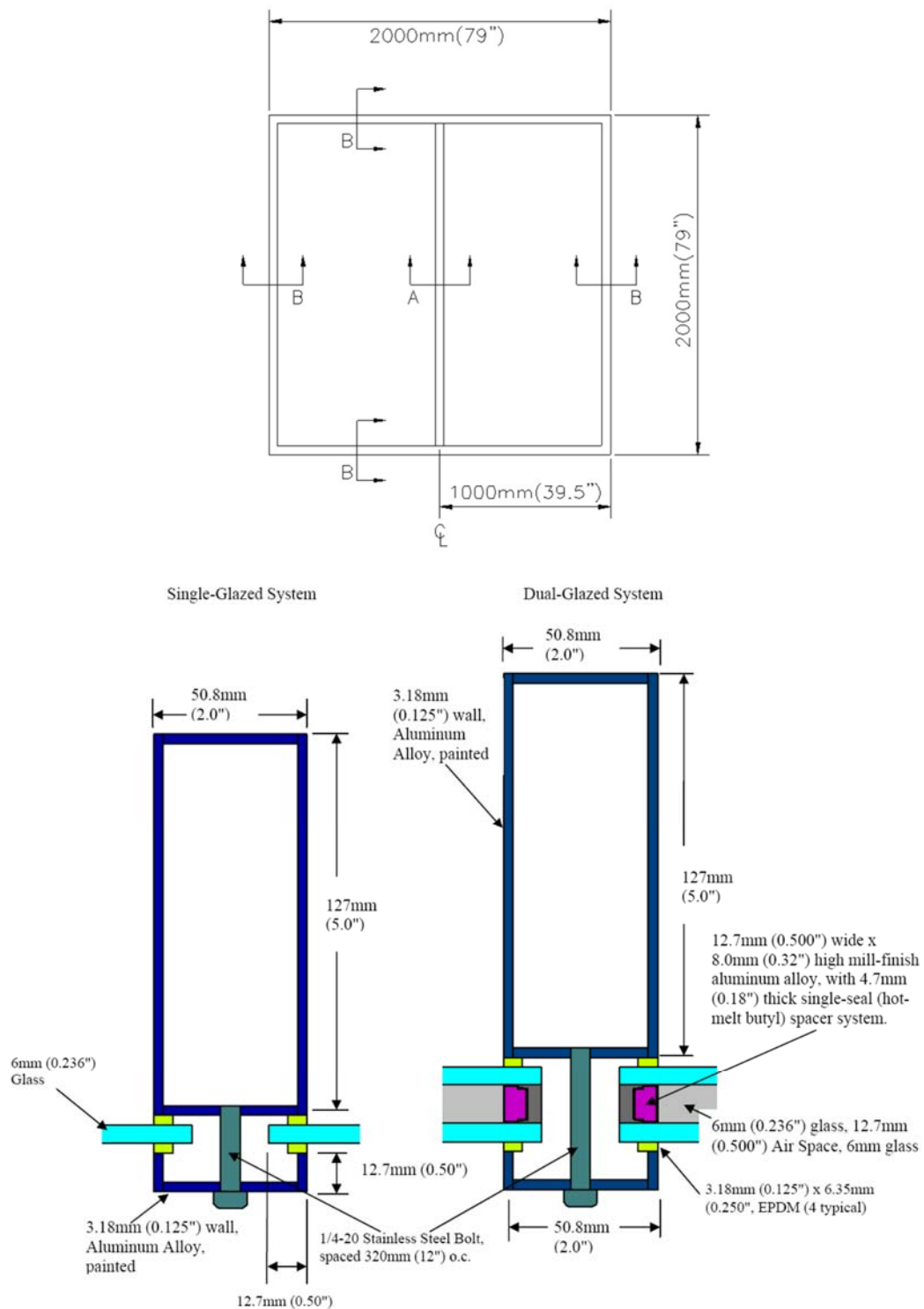
Figure 5-25 – Non-Residential Window-Wall Reference Product
