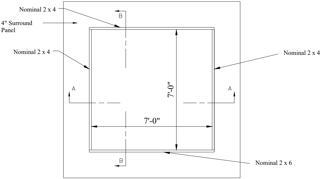
Figure 5-23 – Rolling Door Front Elevation View and Perimeter Details
