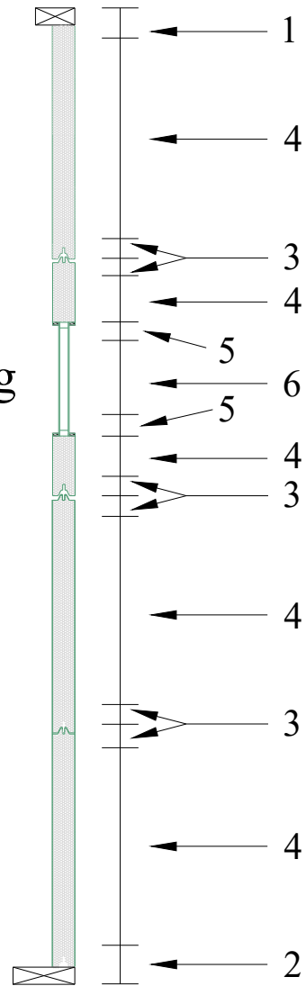
Figure 5-16 – Garage Door U-factor Area Weighting, Sectional
