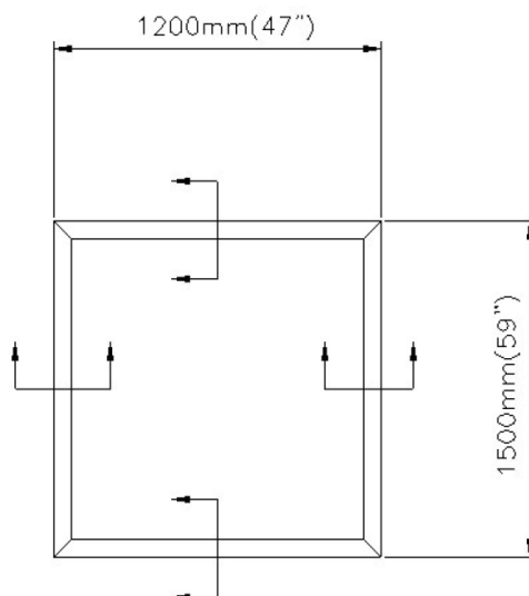
Figure 5-1 Residential Fixed Aluminum Frame Reference Product
