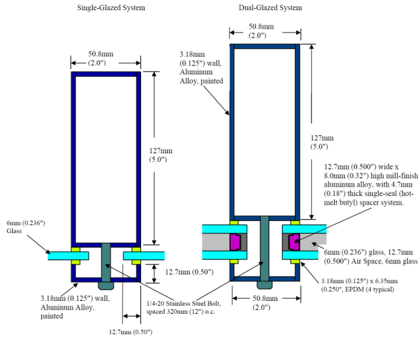
Figure 5-3 Cross Section A
