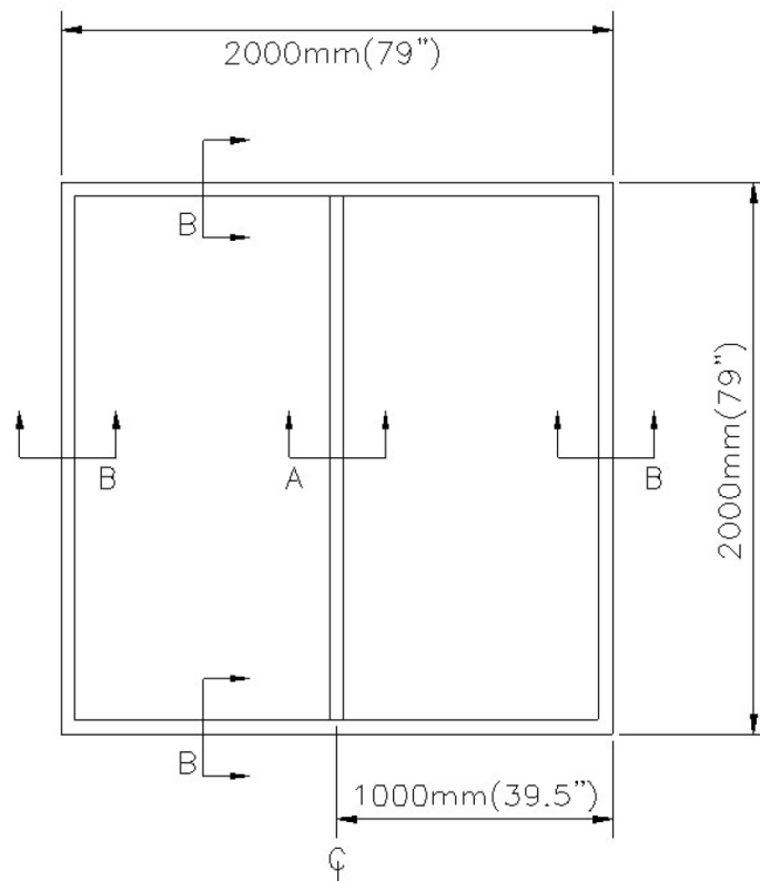
Figure 5-2 Non-residential Windowwall Aluminum Frame Reference Product
