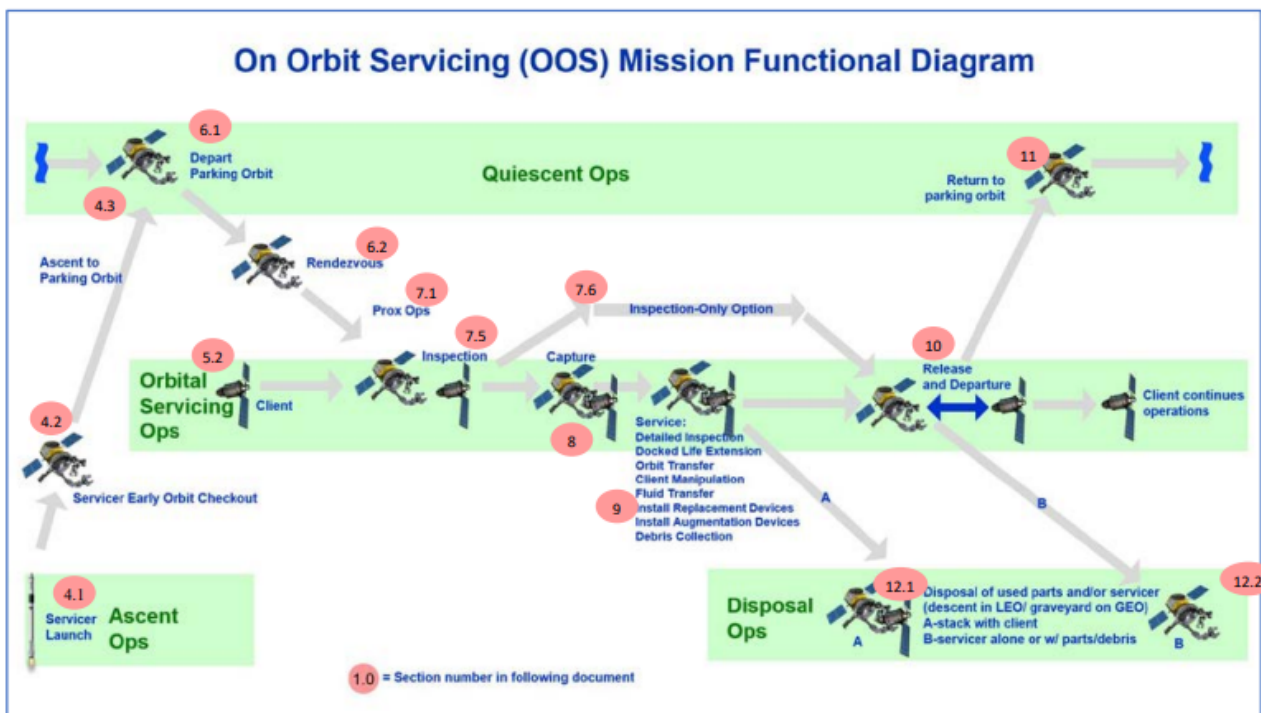
Figure 1 – OOS Mission Functional Diagram
