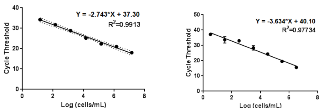
Figure 3. qPCR results of (a) B. bruxellensis and (b) S. cerevisiae . Fluorescence detection cycle threshold values are plotted versus the logarithm of cells/mL.
