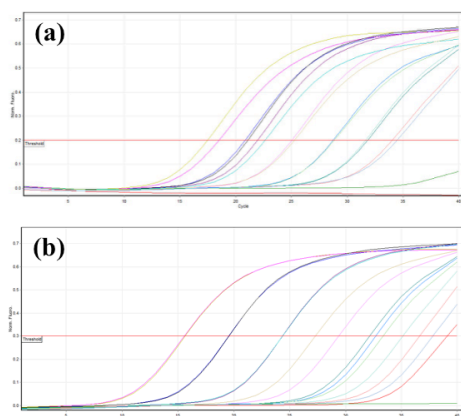
Figure 2. qPCR amplification of (a) B. bruxellensis and (b) S. cerevisiae DNA extracted from 10-fold dilution series, from (a) 1.427 \times 10^7 to 14.27 cells/mL and (b) 3.15 \times 10^6 to 3.15 cells/mL
