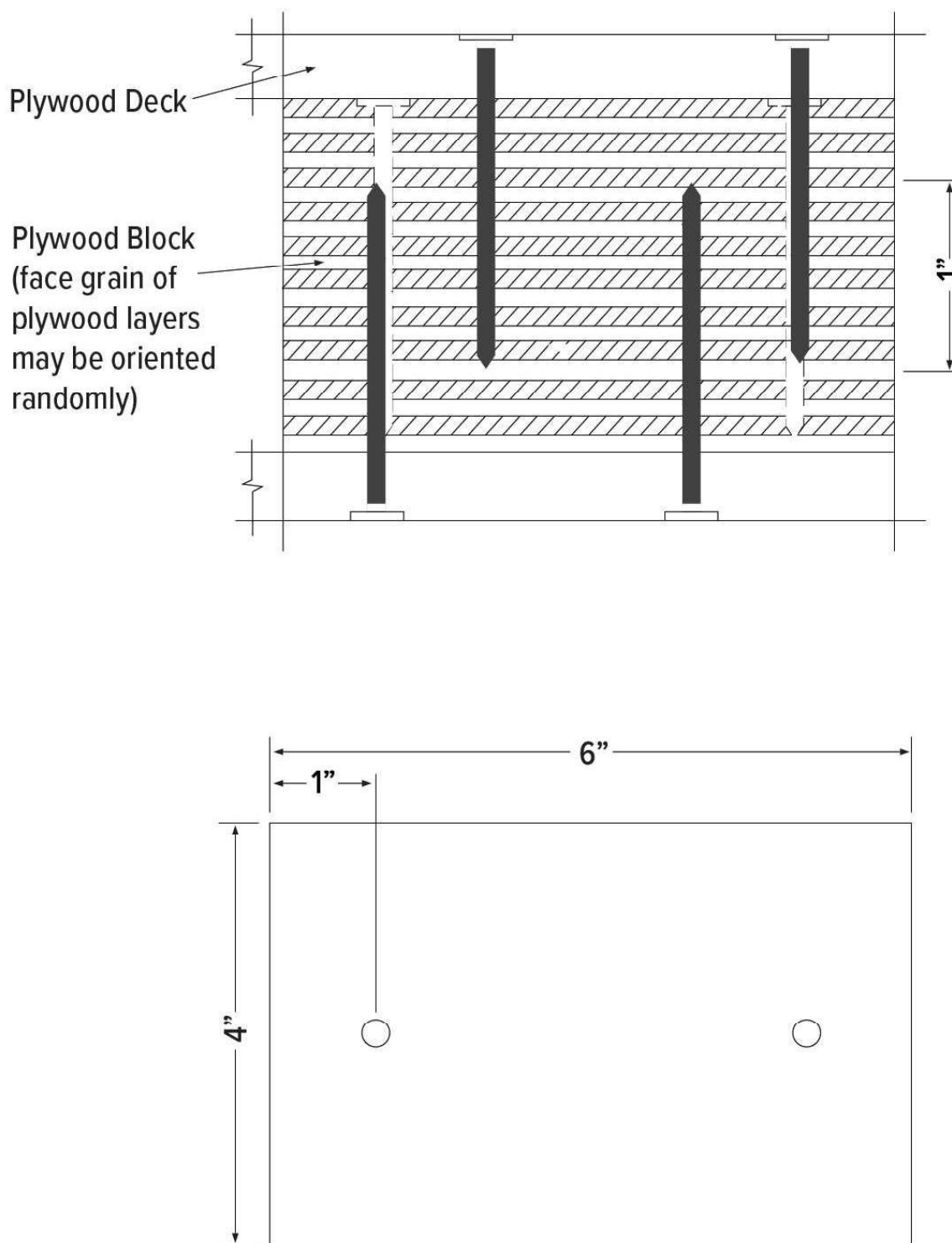
Figure 7. Schematic diagrams of block lamination and fastening.
