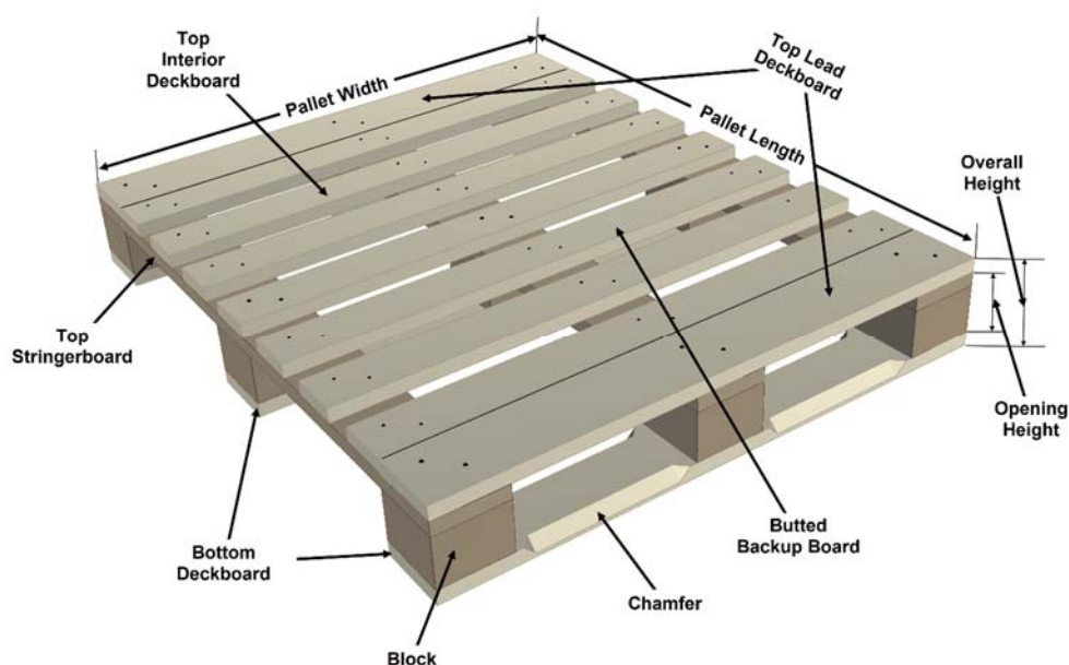
Figure 2. Schematic diagram of a typical block pallet with principal parts labeled.
