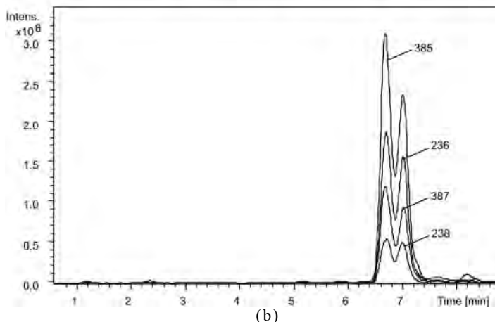
Figure 4. Liquid chromatogram with extracted ion chromatograms for degradation products of fentanyl in trichloroisocyanuric acid aqueous solution over 1 h, showing the (a) \text{M}+\text{H}^+ and (b) \text{M}-\text{H}^+ peaks.
