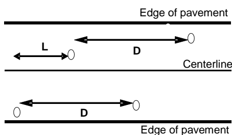
Diagram 1a – Staggered (offset) sampling.
