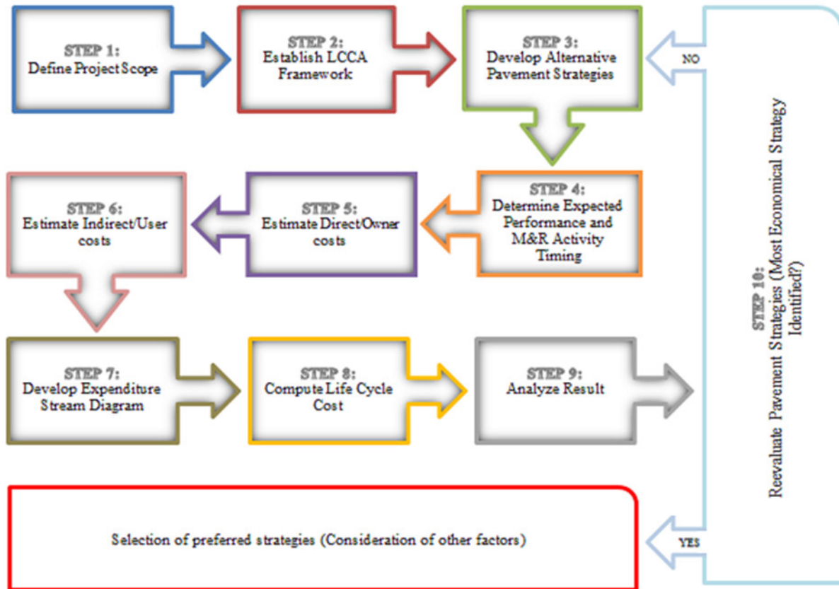
Figure 4- Methodology for conducting airport/highway pavement LCCA
