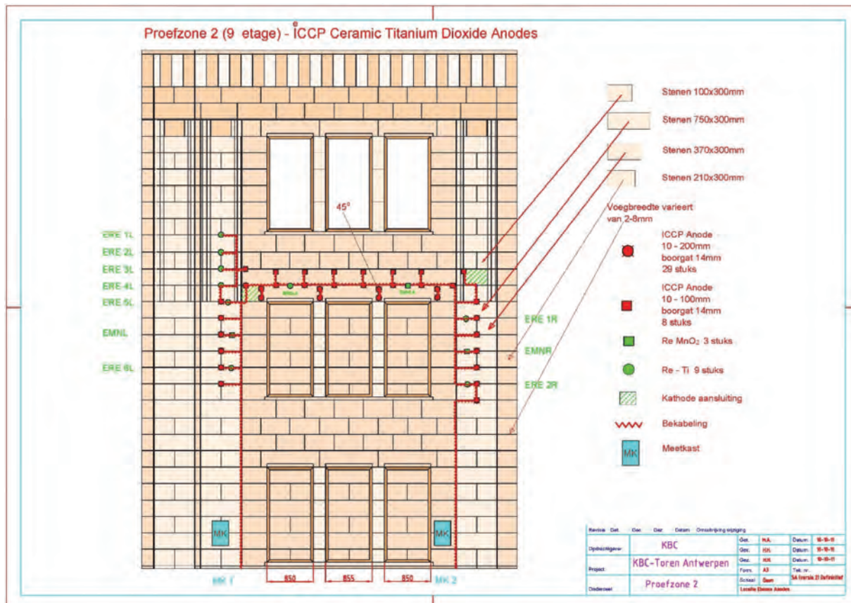
Fig. 8: ICCP anode layout
