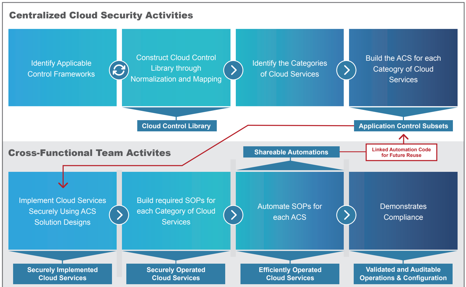
Visual representation of the BreakFree Cloud Security Framework.
