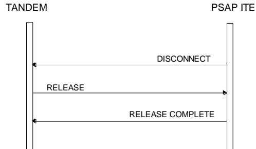
FIGURE 5.3 --ISDN Call disconnect when initiated by the ISDN PSAP
