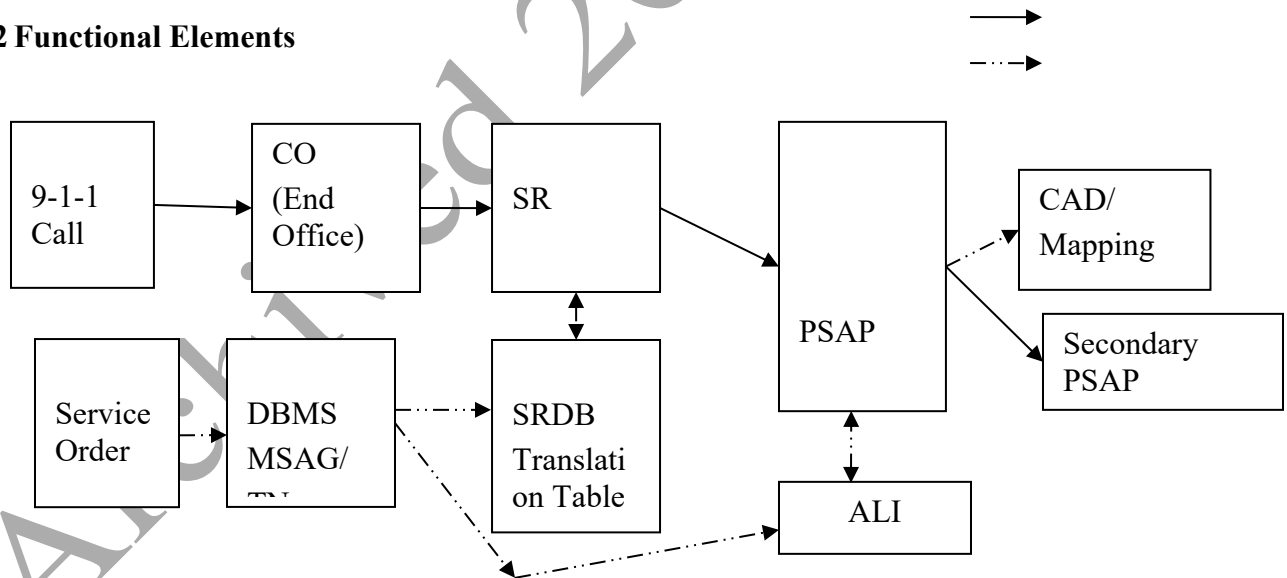
Figure 12-6 Legacy Baseline – Wireline/Legacy/Enhanced 9-1-1
