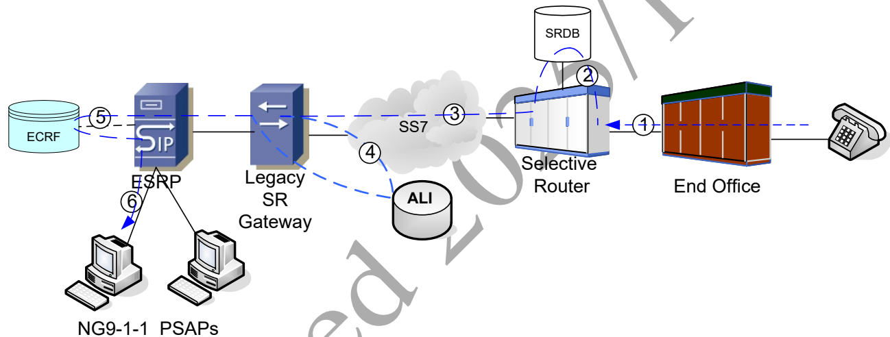
Figure 8-2 Wireline Call Transiting Selective Router to NG9-1-1 System
