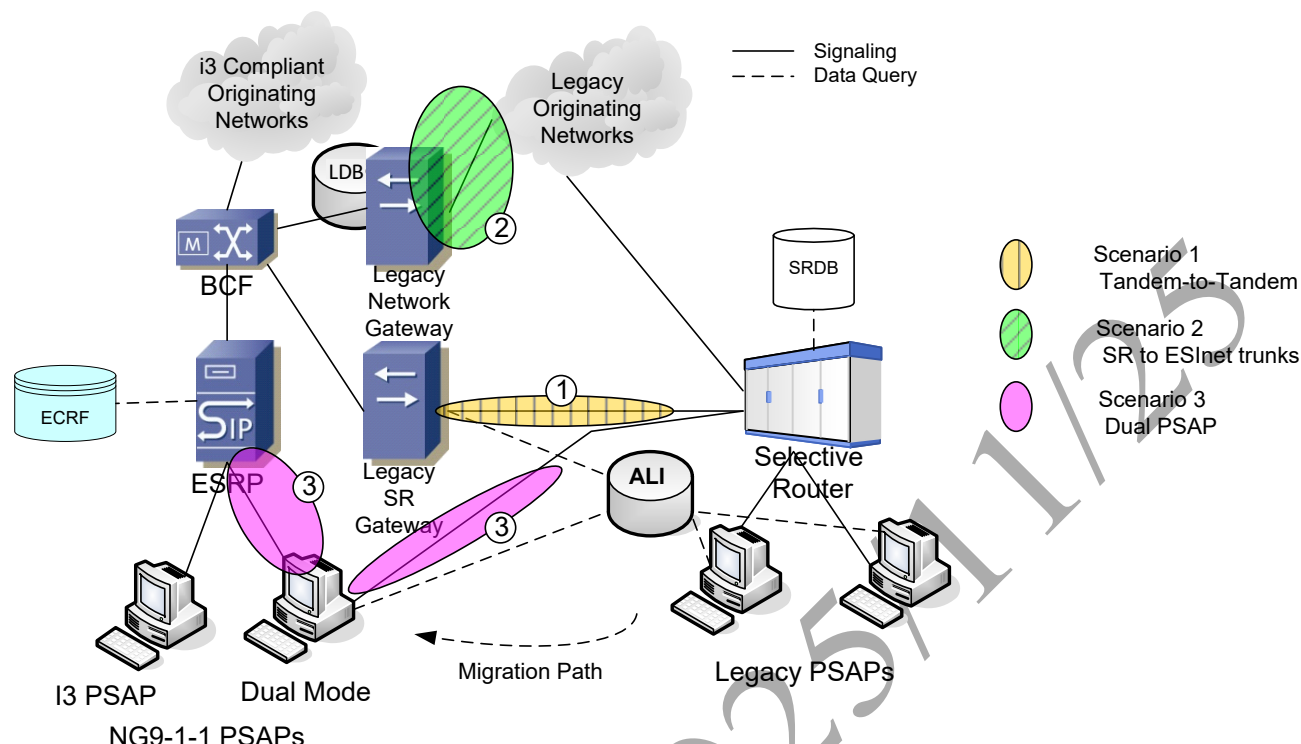
Figure 8-1 Transition Reference Model
