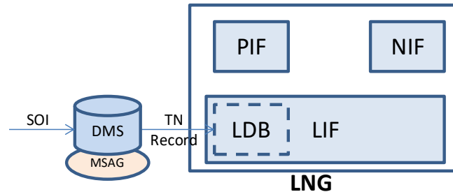
Figure 11-5 LDB Provisioning via the Database Management System
