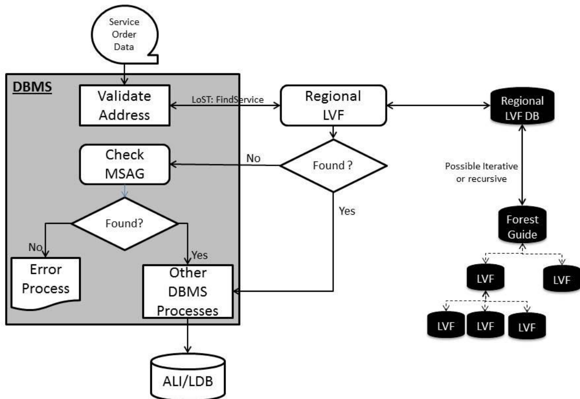
Figure 11-1 Civic Address Validation During Transition
