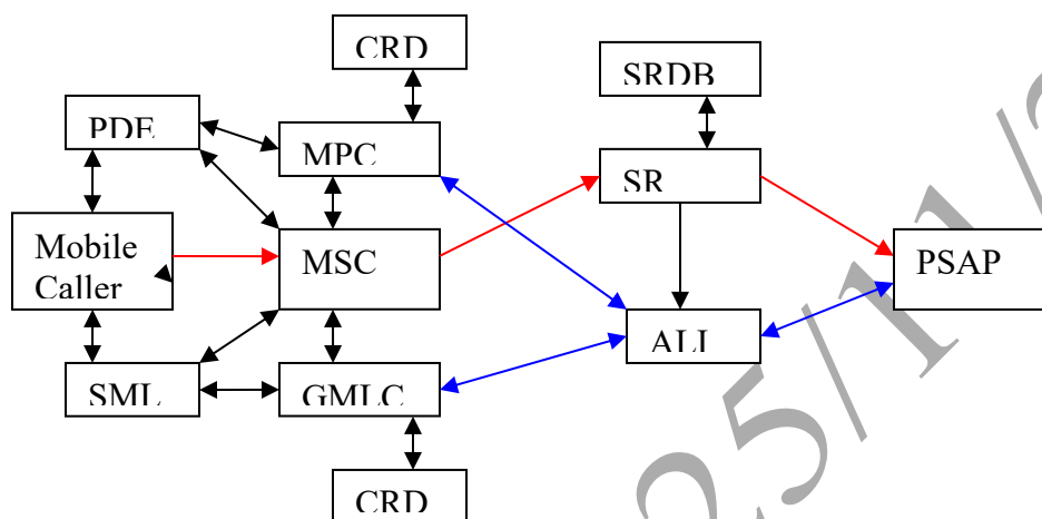
Figure 12-10 Legacy Baseline – Wireless/Legacy/Phase II - 2
