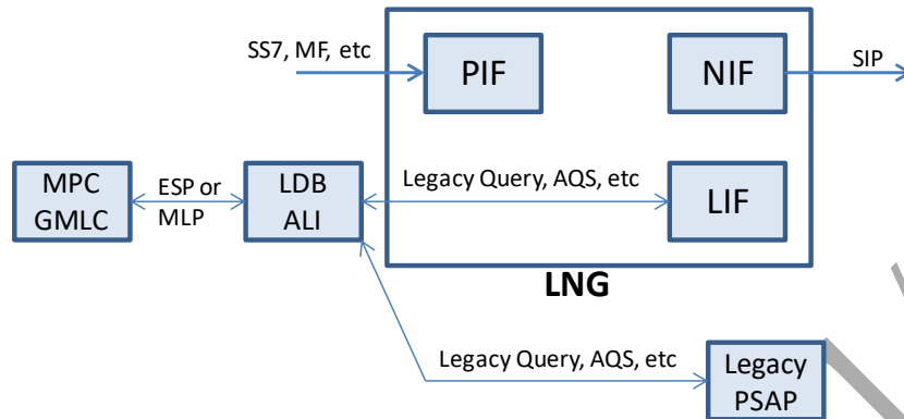
Figure 11-3 LDB as Legacy ALI
