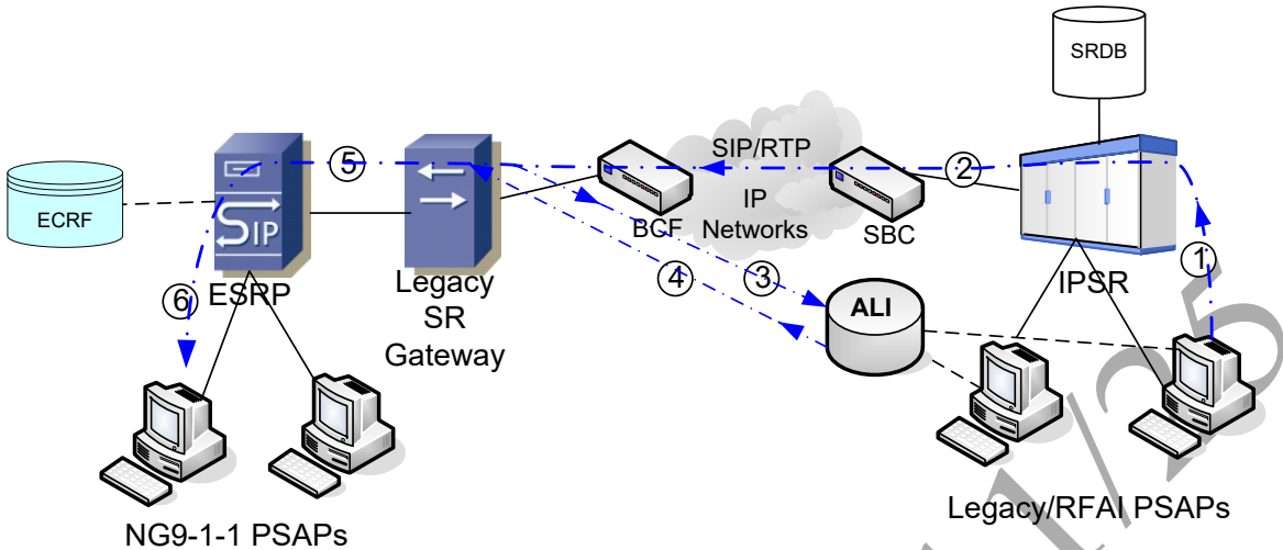
Figure 10-4 Bridging from IPSR to i3 Network
