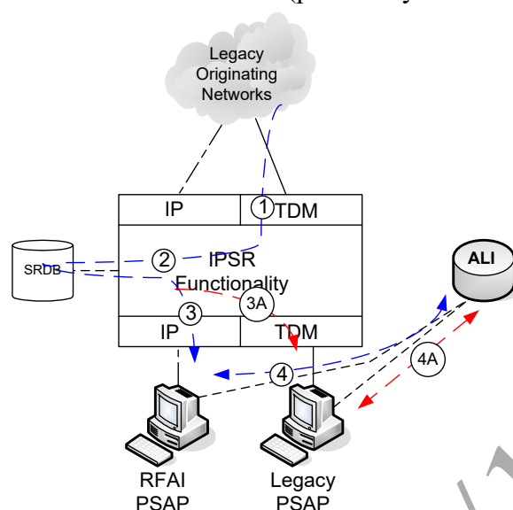
Figure 10-2 IPSR Call Flow
