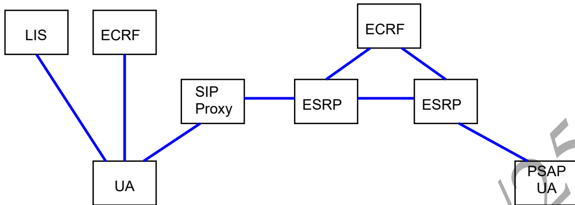
Figure 12-15 Next Generation 9-1-1 Baseline – Event Notification
