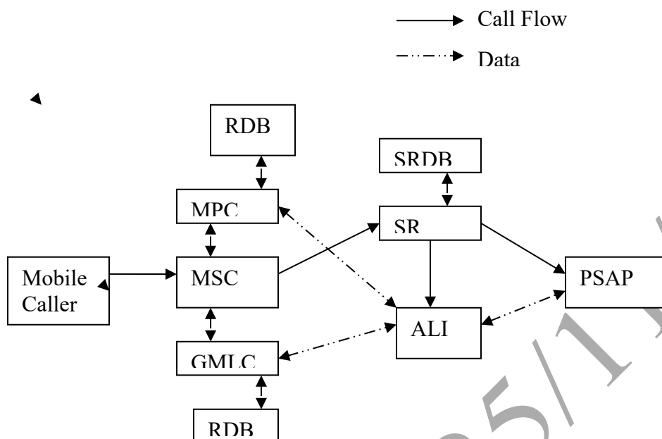
Figure 12-8 Legacy Baseline – Wireless/Legacy/Phase 1
