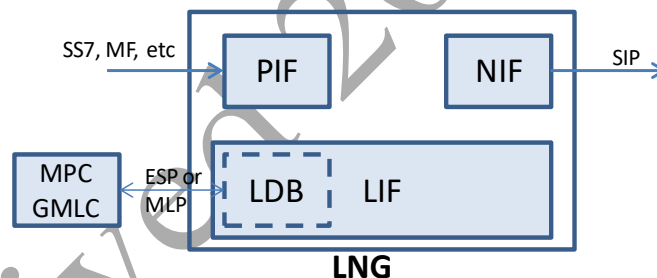
Figure 11-4 LDB integrated into the LNG
