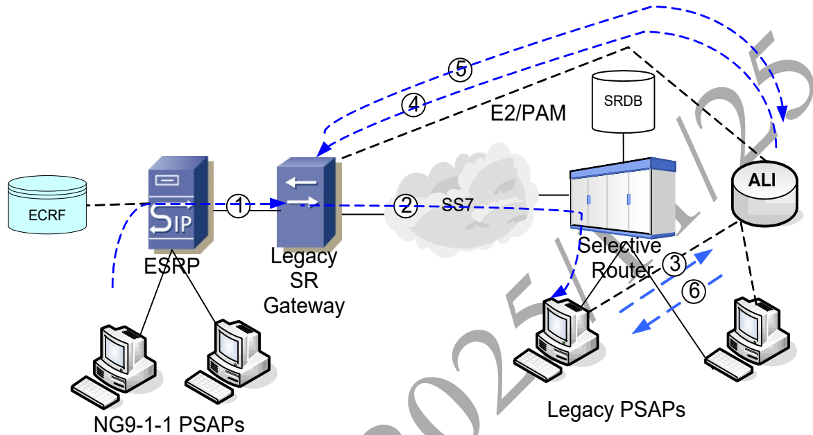
Figure 8-5 Bridge – NG9-1-1 PSAP to Legacy PSAP
