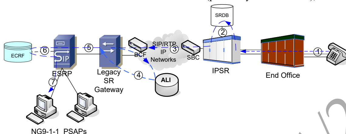
Figure 10-3 Initial Call Routed via IPSR
