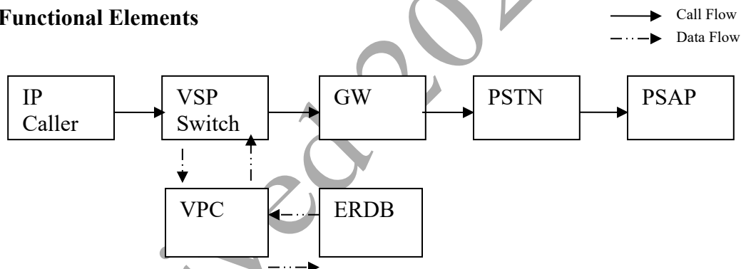
Figure 12-5 Legacy Baseline – Wireline/IP/Basic 9-1-1
