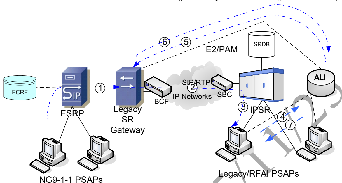
Figure 10-5 Bridging from an i3 Network to the IPSR
