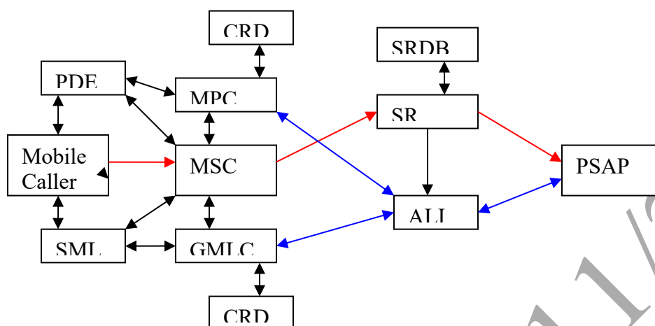
Figure 12-9 Legacy Baseline – Wireless/Legacy/Phase II
