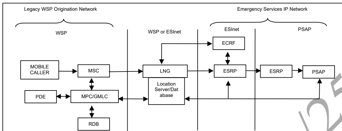
Figure 12-16 Next Generation 9-1-1 Baseline – Legacy Wireless (Origination)
