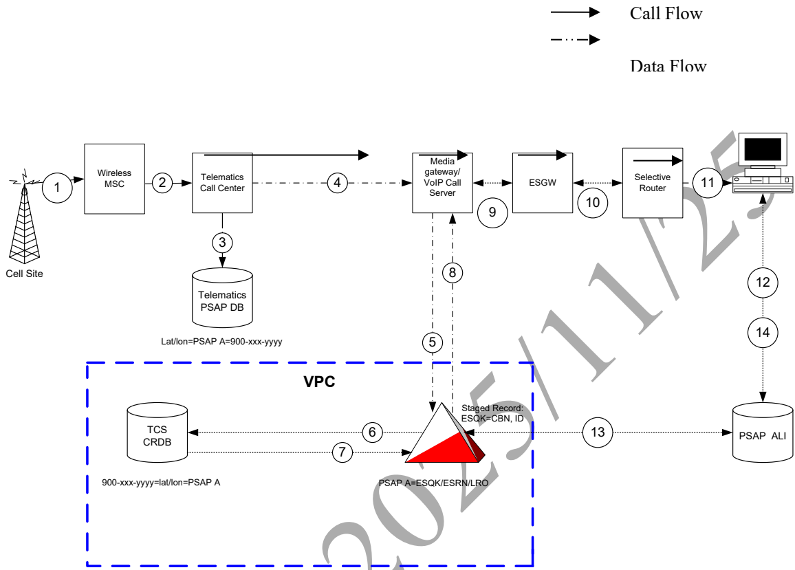
Figure 12-13 Legacy Baseline – 3 Party Relay Calls 2c
