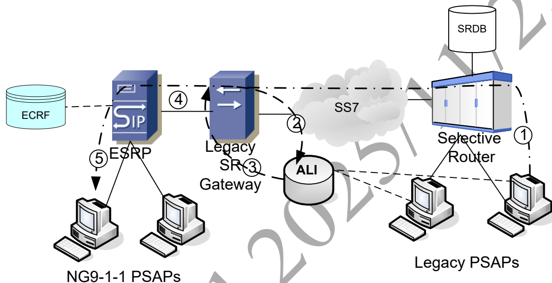
Figure 8-4 Bridge – Legacy PSAP to NG9-1-1 PSAP
