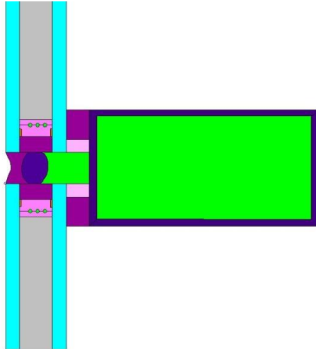
Figure 2: Silicone structural glazed system
