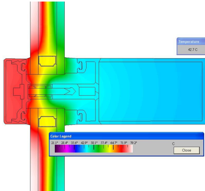
Figure 5: Therm results for a dry glazed system with clear insulating glass and an aluminum IG spacer at an exterior temperature of 50C and 1120 W/m 2 solar load noting a 42.7 C frame temperature
