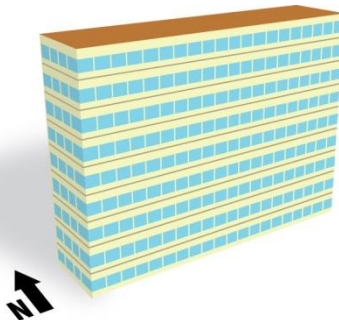
Figure 6: 12m x 50m x 9 story building model for energy analysis
