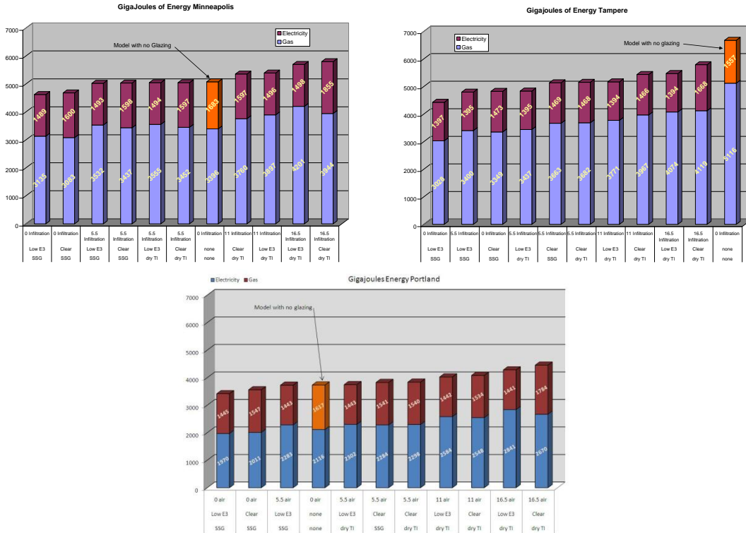
Figure 8: Energy Use of a 9 Story Building in a Cold Climate: Portland, OR; Minneapolis, MN and Tampere, Finland with variations on IG, system design and air infiltration rates
