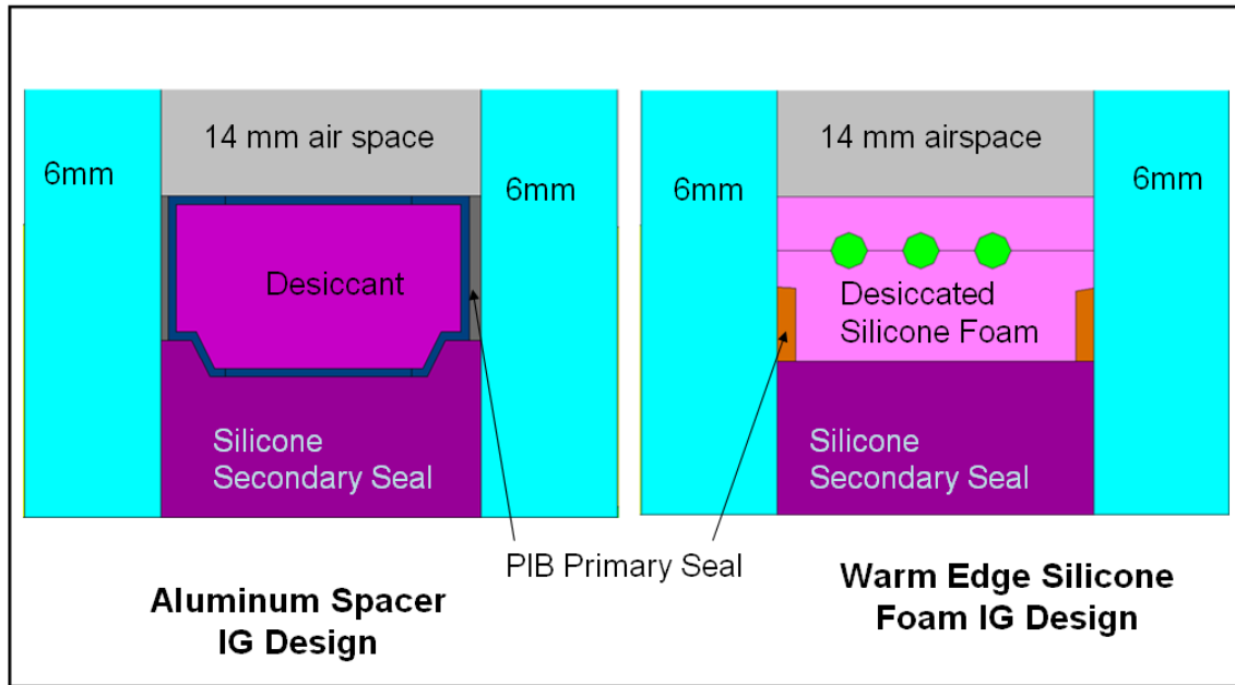
Figure 3: Configuration of the two types of insulating glass
