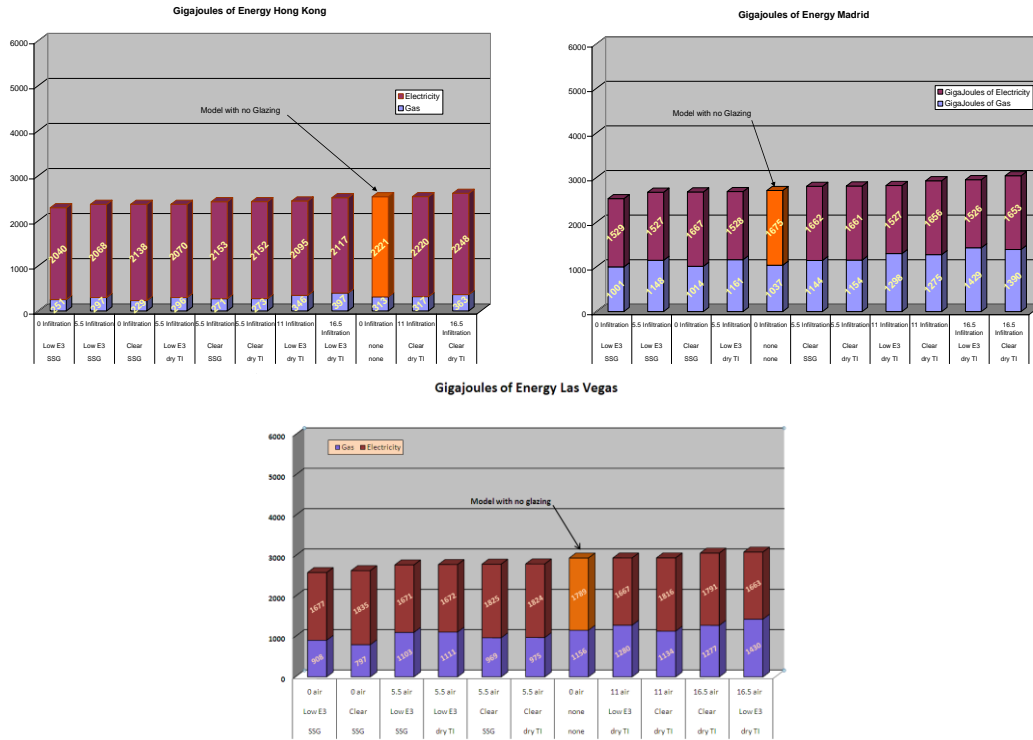
Figure 7: Energy Use of a 9 story building in a Hot Climate, Hong Kong, Madrid Spain and Las Vegas Nevada with variations on IG, system design and air infiltration rates
