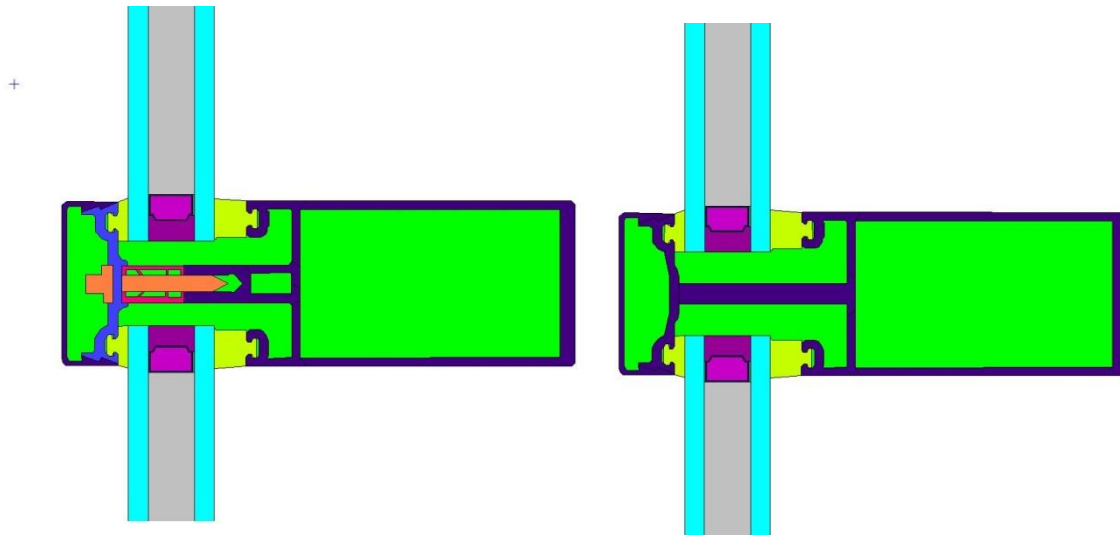
Figure 1: Dry glazed thermally improved system (left) and non-broken dry glazed aluminum system (right)
