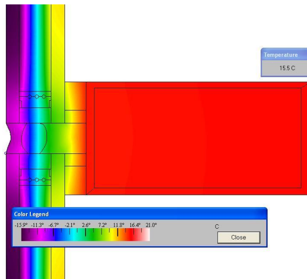
Figure 4: Therm Results for Structural silicone glazed system using high performance glass and a silicone foam warm edge IG spacer at -18C exterior and 21C interior noting a 15.5C frame temperature
