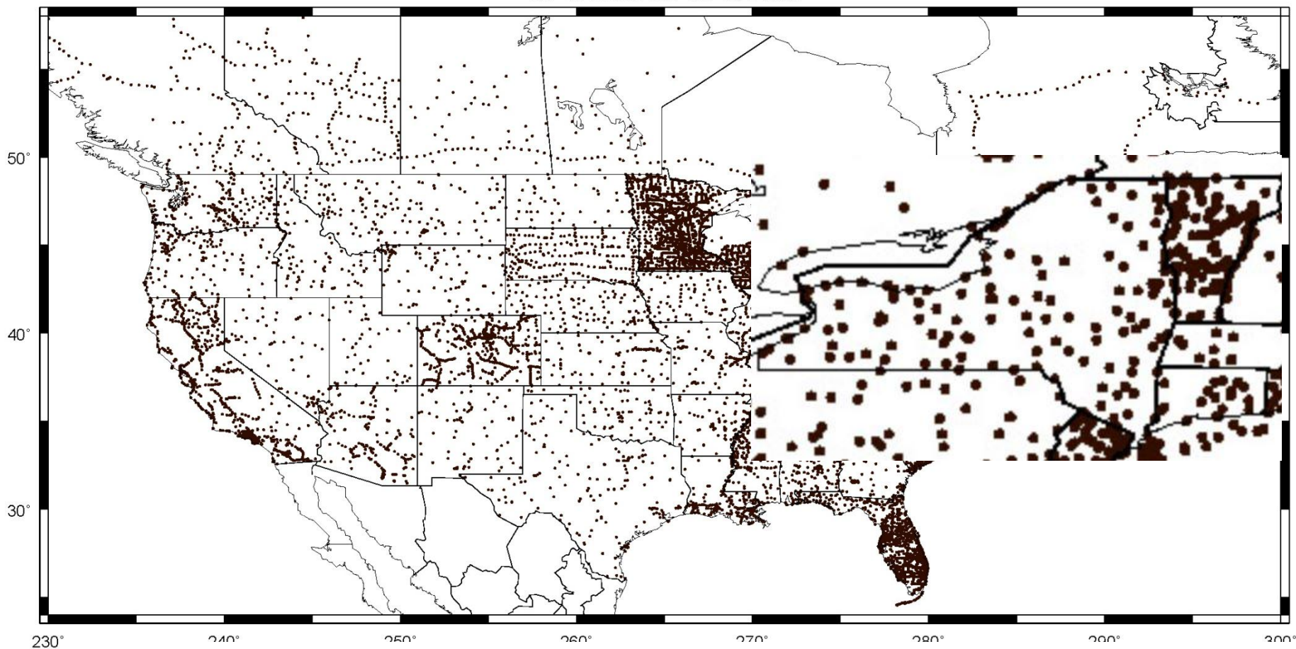
GPS BMs for GEOID09
