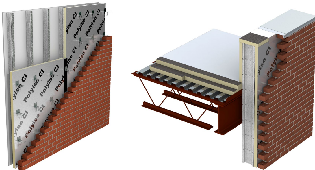
Figure 3: Typical assemblies with polyiso wall insulation boards installed in framed wall (left image) and mass wall (right image).
