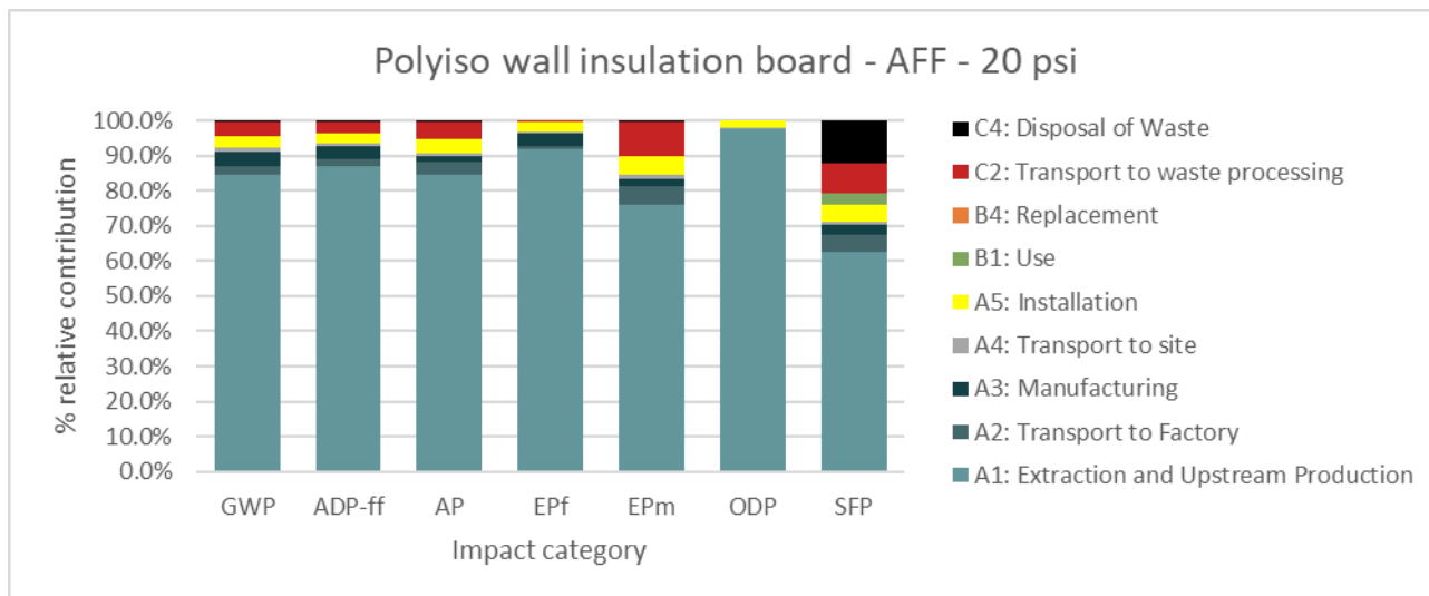
Figure 7: Contribution of life cycle information modules to the potential environmental impacts of 1m 2 of installed polyiso wall insulation board, AFF, 20 psi, for 75 years.
