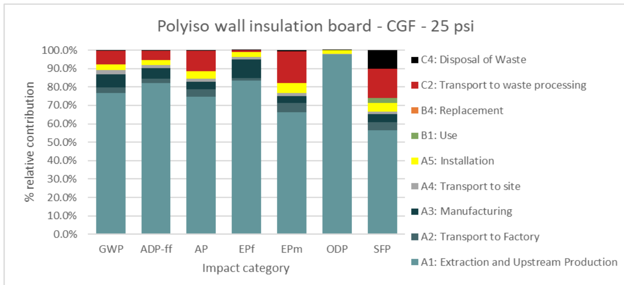
Figure 11: Contribution of life cycle information modules to the potential environmental impacts of 1m 2 of installed polyiso wall insulation board, CGF, 25 psi, for 75 years.
