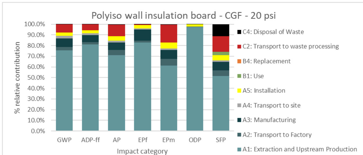
Figure 10: Contribution of life cycle information modules to the potential environmental impacts of 1m 2 of installed polyiso wall insulation board, CGF, 20 psi, for 75 years.
