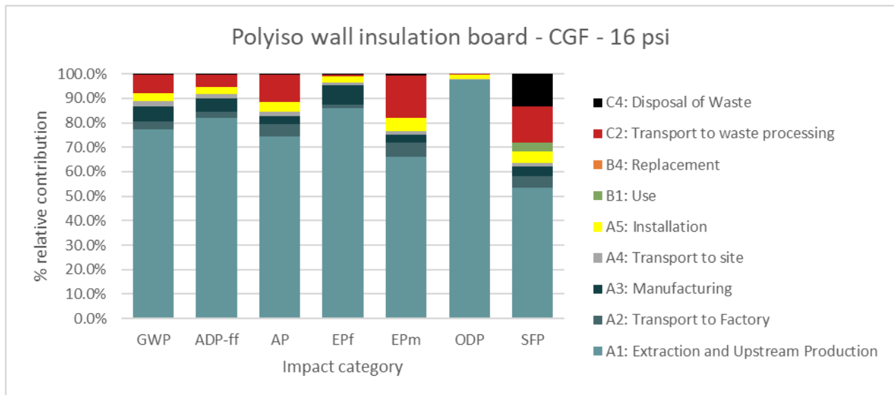
Figure 9: Contribution of life cycle information modules to the potential environmental impacts of 1m 2 of installed polyiso wall insulation board, CGF, 16 psi, for 75 years.
