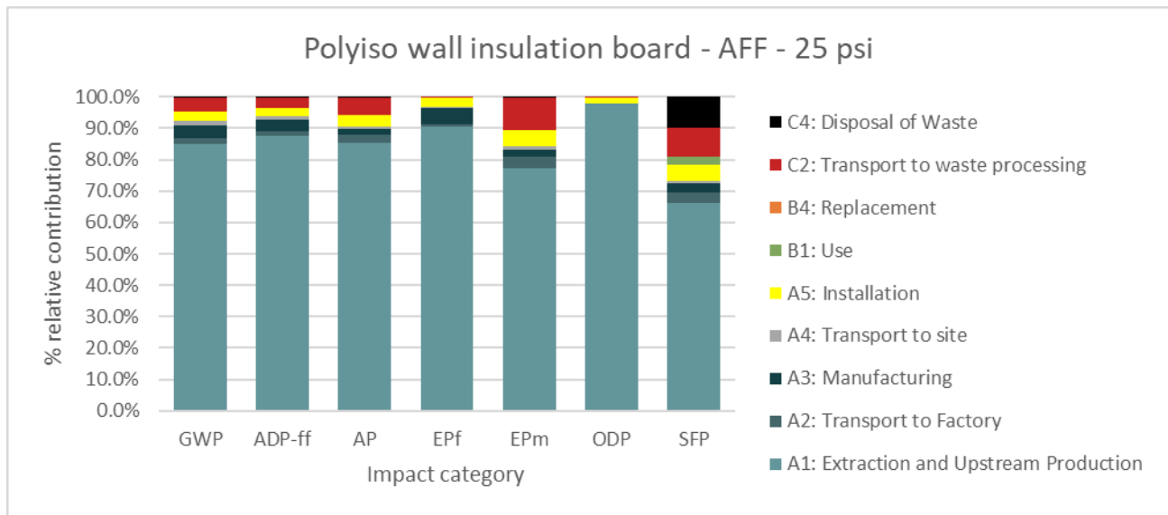
Figure 8: Contribution of life cycle information modules to the potential environmental impacts of 1m 2 of installed polyiso wall insulation board, AFF, 25 psi, for 75 years.
