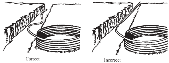
Figure 2: Correct and incorrect snaking
