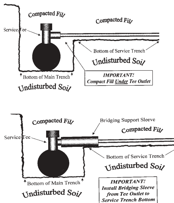
Figures 4 (below) & 5(botton): Connecting PE to a tap or other rigidly held structure.
