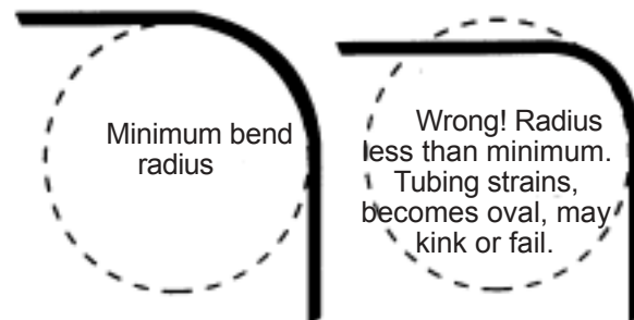
Figure 3: Bending radius of PE pipe.
