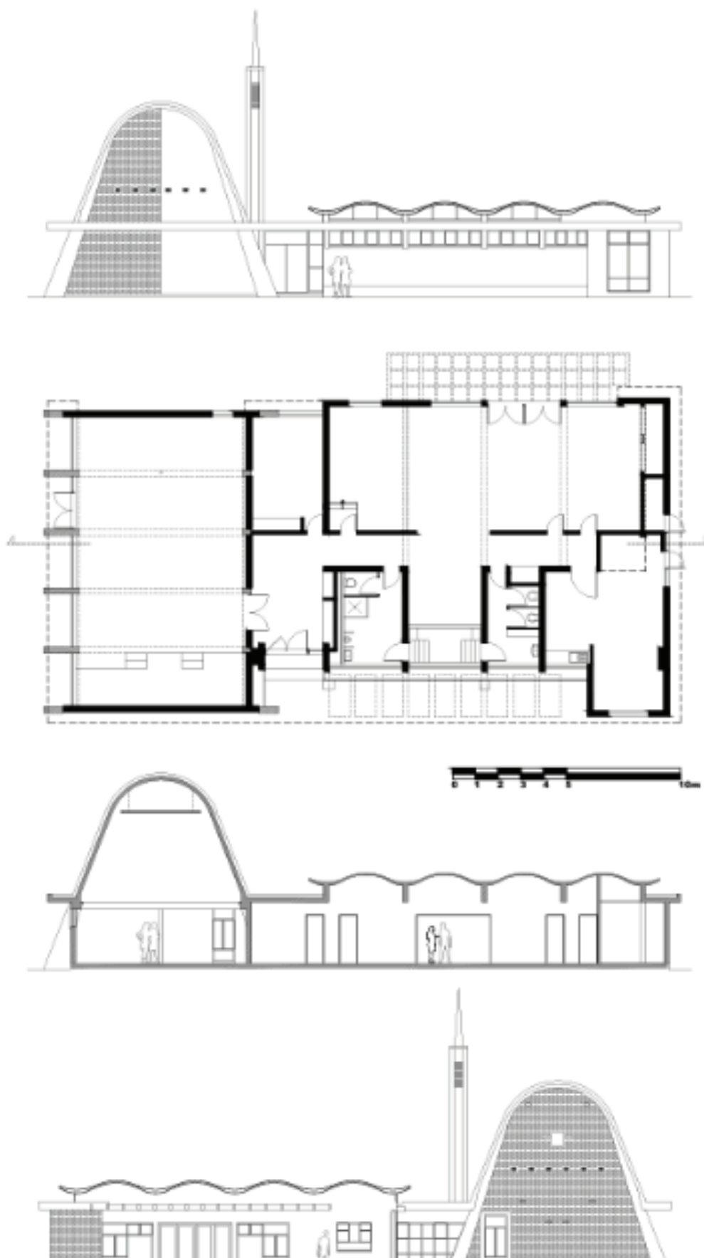
Figure 4 Diagram of Architectural Features of the Chapel, Indicating the South Elevation, Plan, Basic Section and North Elevation, AutoCAD Drawings by Raubenheimer, 2013, and Redrawn by Odendaal, 2025. [Not to scale]
