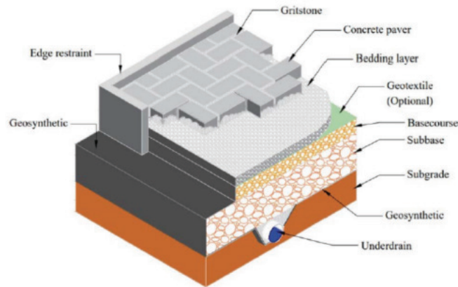
Figure 1 Typical PICP Section (Monyake & Armitage 2023)
