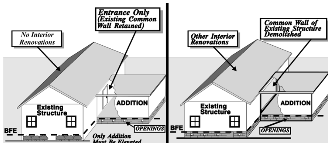
Figure 8-4. Lateral additions to a residential building in an A Zone.
